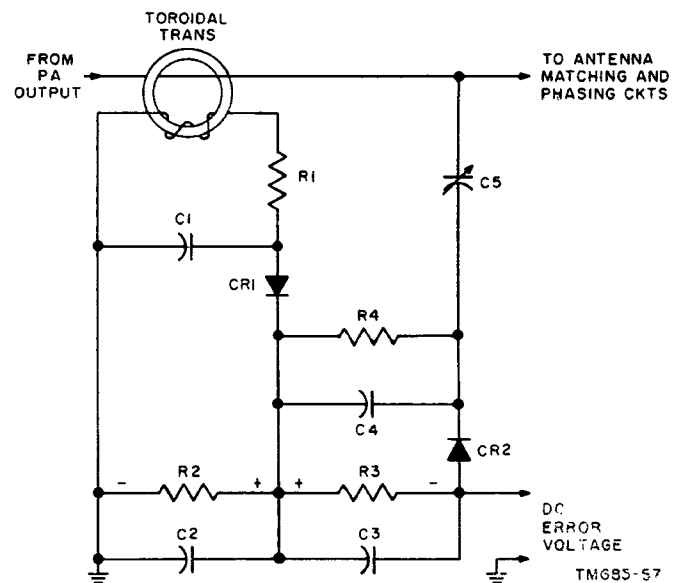
Figure 57. Impedance error detector, schematic diagram.
