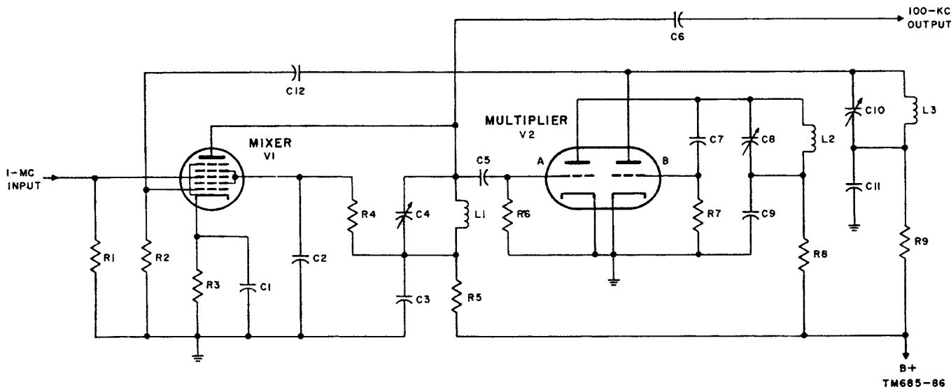
Figure 86. Regenerative frequency divider, schematic diagram
