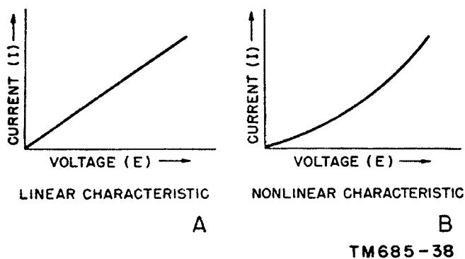
Figure 38. Voltage-current characteristics.
