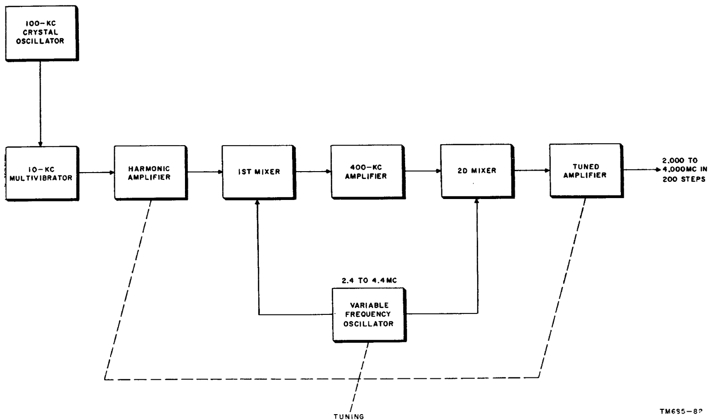
Figure 82. Single-crystal frequency synthesizer using superheterodyne principle, block diagram.
