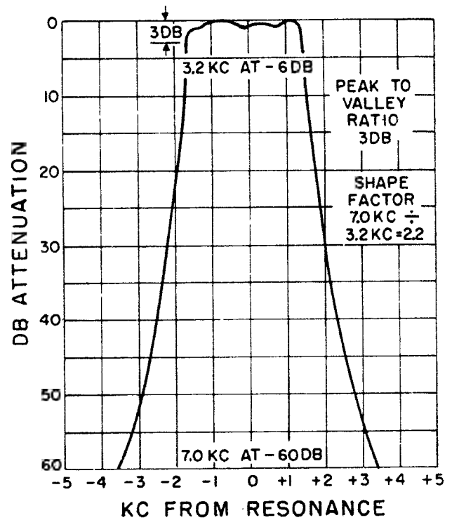
Figure 27. Mechanical filter, characteristic curve.
