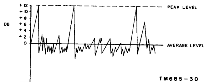
Figure 30. Peak-to-average level variations of speech.
