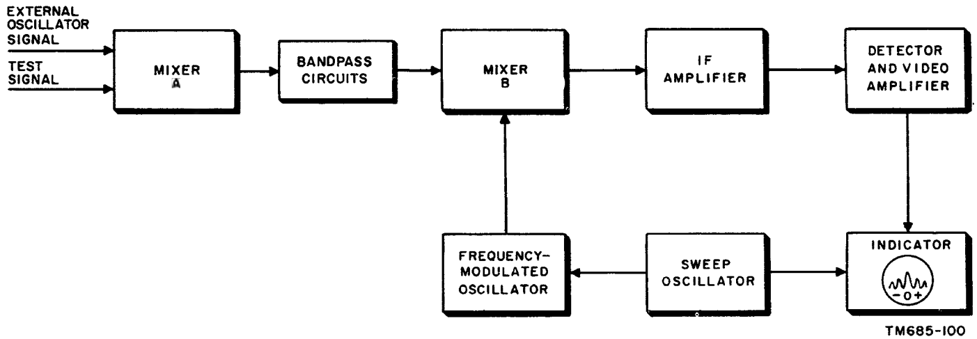
Figure 100. Panoramic indicator, simplified block diagram.
