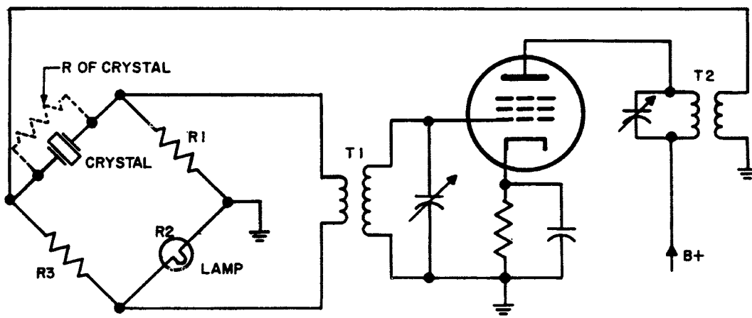
Figure 78. Bridge-stabilized crystal oscillator circuit.
