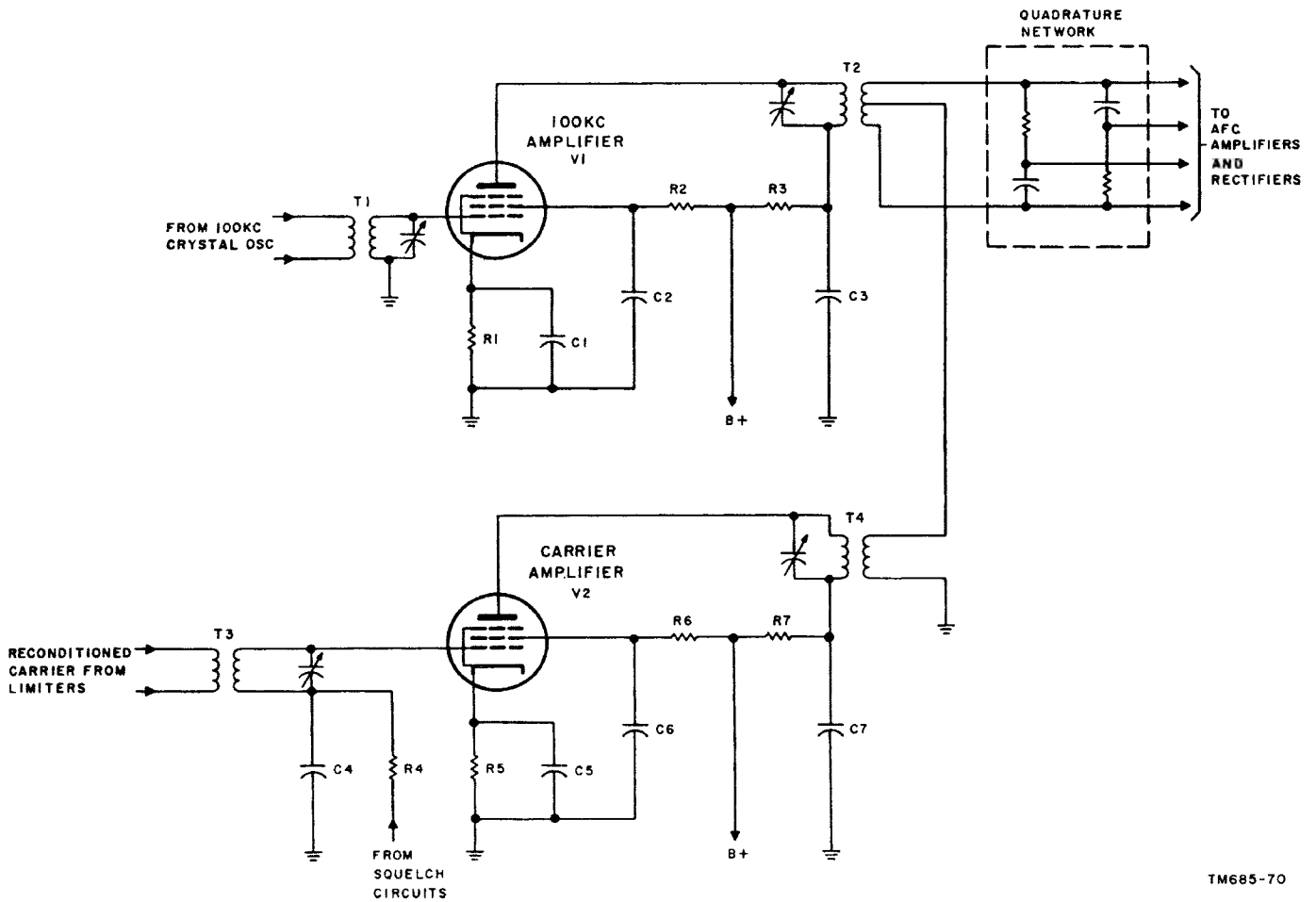
Figure 70. Carrier amplifier and 100-kc amplifier, schematic diagram.
