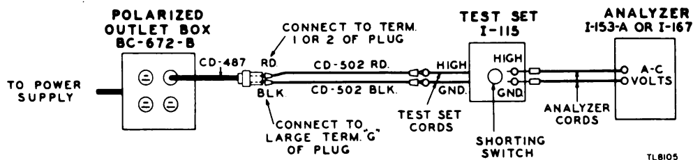
Figure 29. Test Set I-115, sketch of test connections.
