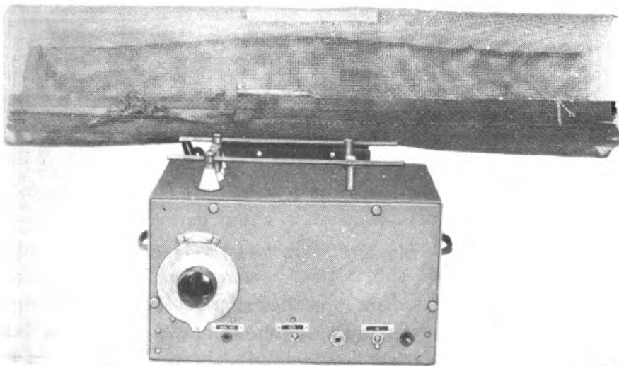
Figure 8. Radio Modulator BC-423-B, front view.
