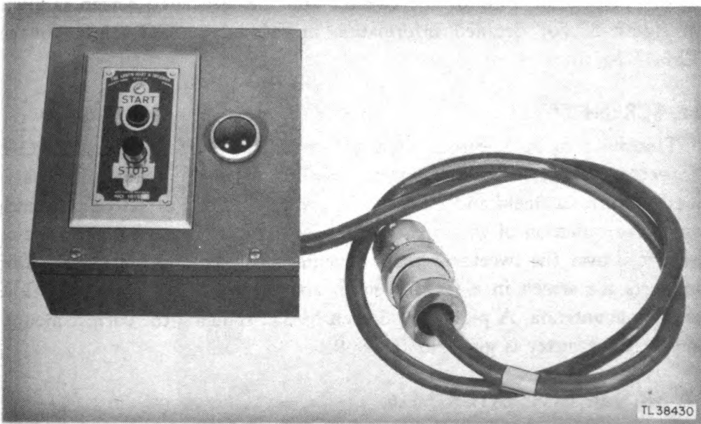
Figure 5. Remote Control Box BC-670-B, front view.
