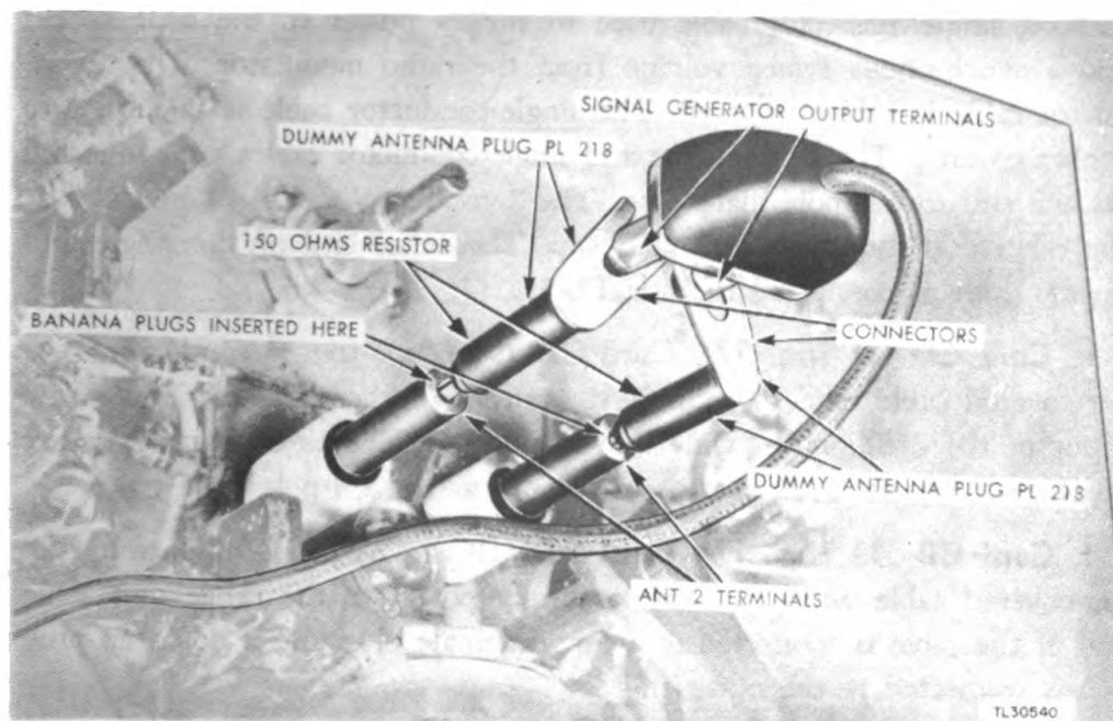
Figure 16. Plug PL-218, sketch.
