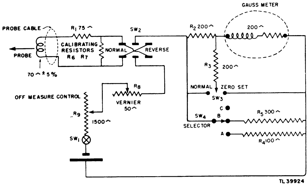
Figure 35. Fluxmeter TS-15A/AP, schematic diagram.
