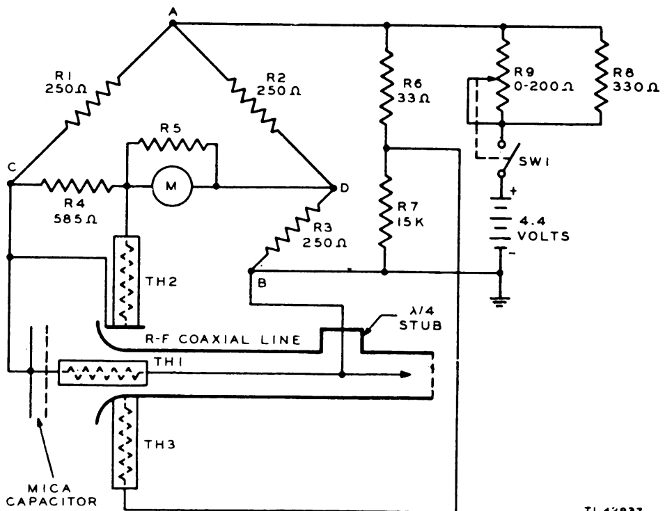
Figure 36. Power Meter TS-125/AP, schematic diagram.
