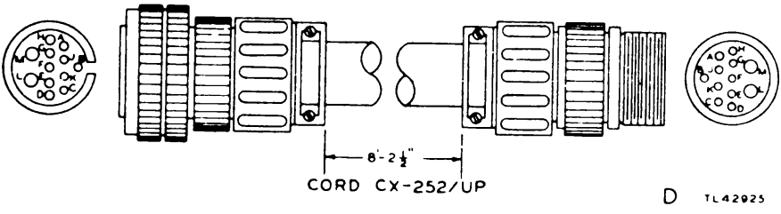
Figure 15. Details of Cords CX-249/UP, CX-250/UP, CX-251/UP, and CX-252/UP.
