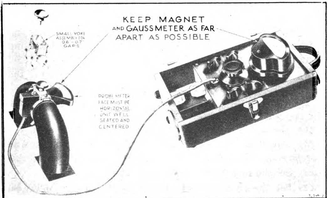
Figure 30. Use of Fluxmeter TS-15A/AP.
