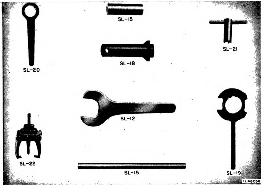
Figure 25. Tools used with Test Set AN/MPM-2.
