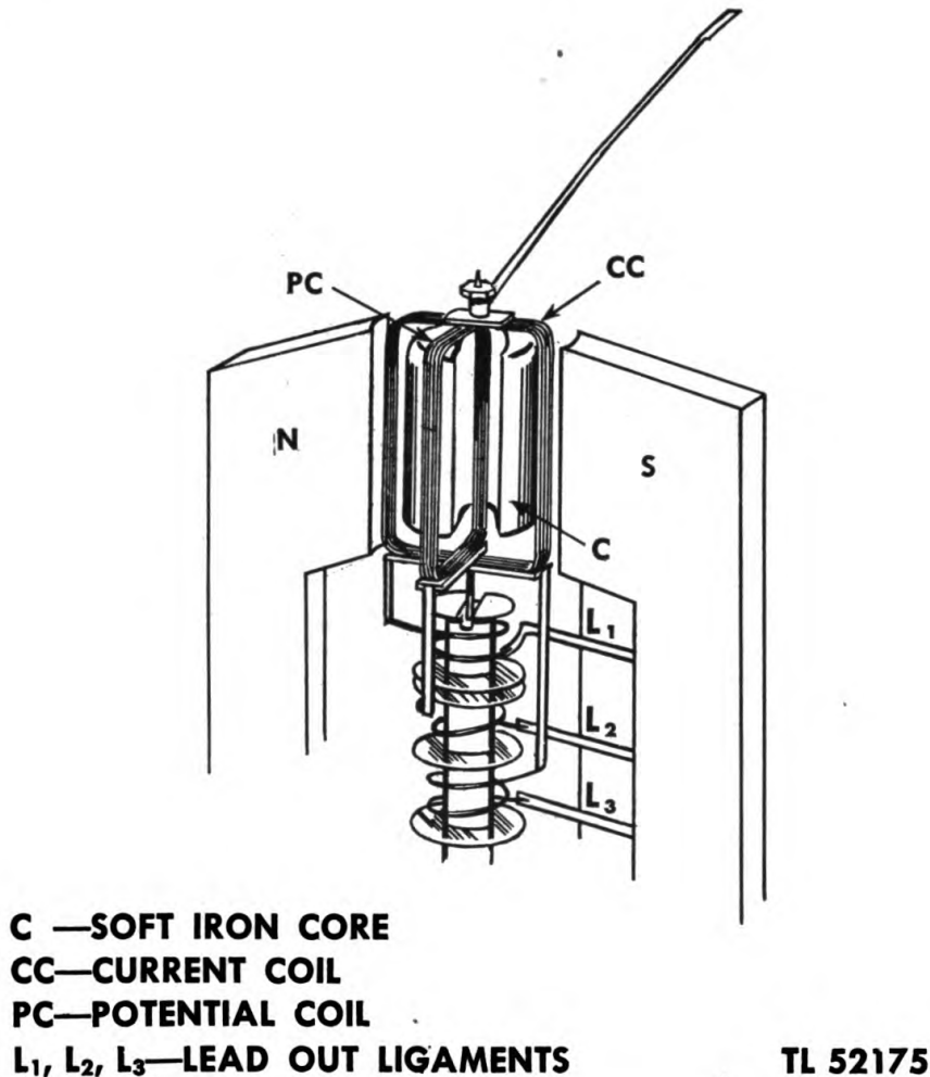
Figure 8. Ohmmeter movement of Test Set I-48-B.
