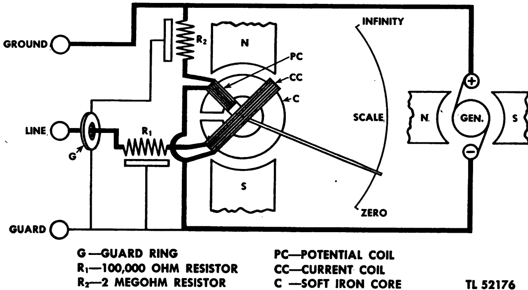
Figure 9. Test Set I-48-B, schematic diagram.
