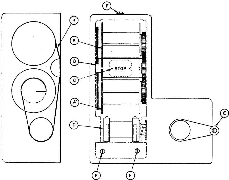
Figure 10—Dial mechanism
