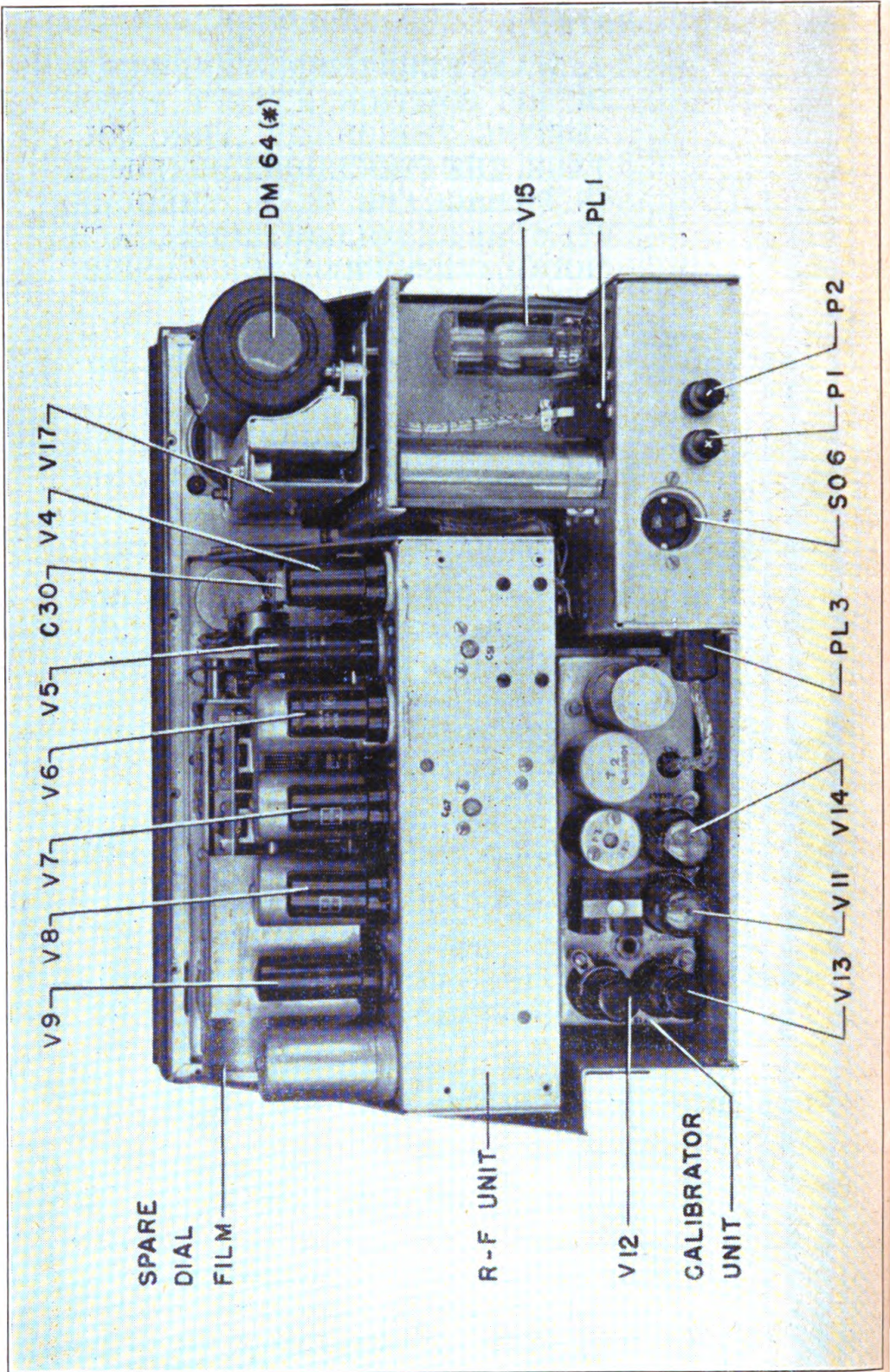
Figure 7A—Revised Signal Generator I-208A, rear view, dust cover removed
