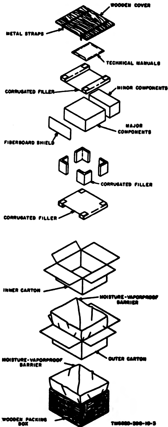
Figure 2-1. Typical packaging.
