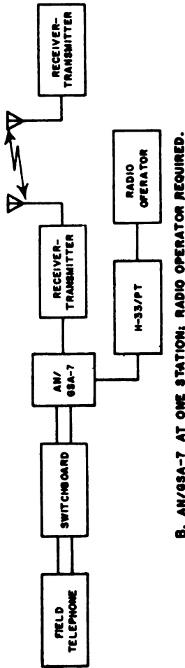
A. AN/GSA-7 AT BOTH STATIONS; RADIO OPERATOR NOT REQUIRED.
