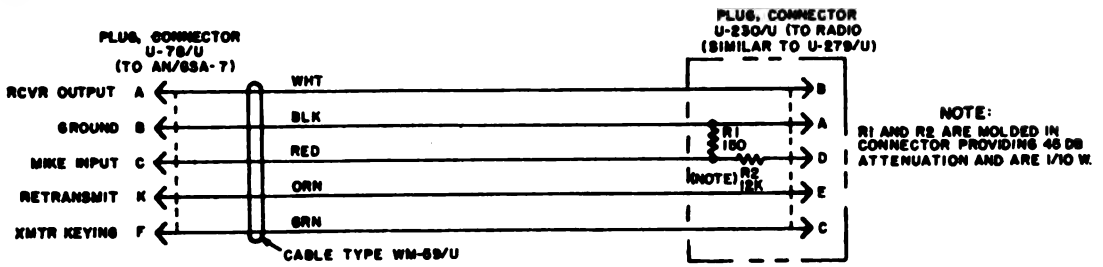
B. CABLE ASSEMBLY, SPECIAL PURPOSE, ELECTRICAL CX-7474/U.
