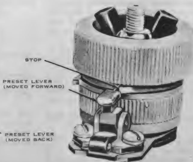
C. TUNING CONTROL; STOP AGAINST PRESET LEVER.
