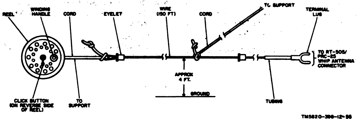
Figure 6-8. Antenna AT-884A/G, installation and parts.
