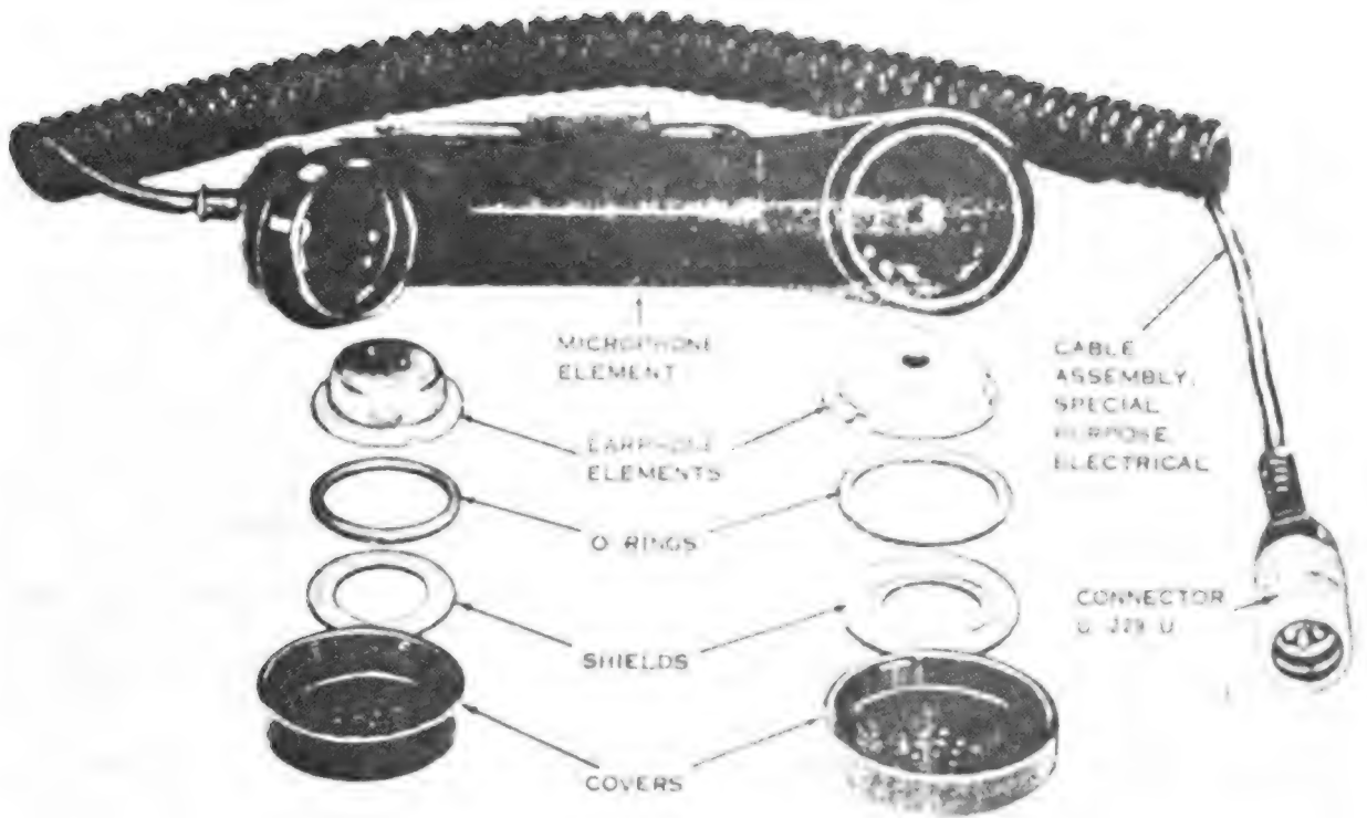
Figure 1-8. Handset H-189/GR, disassembled.
