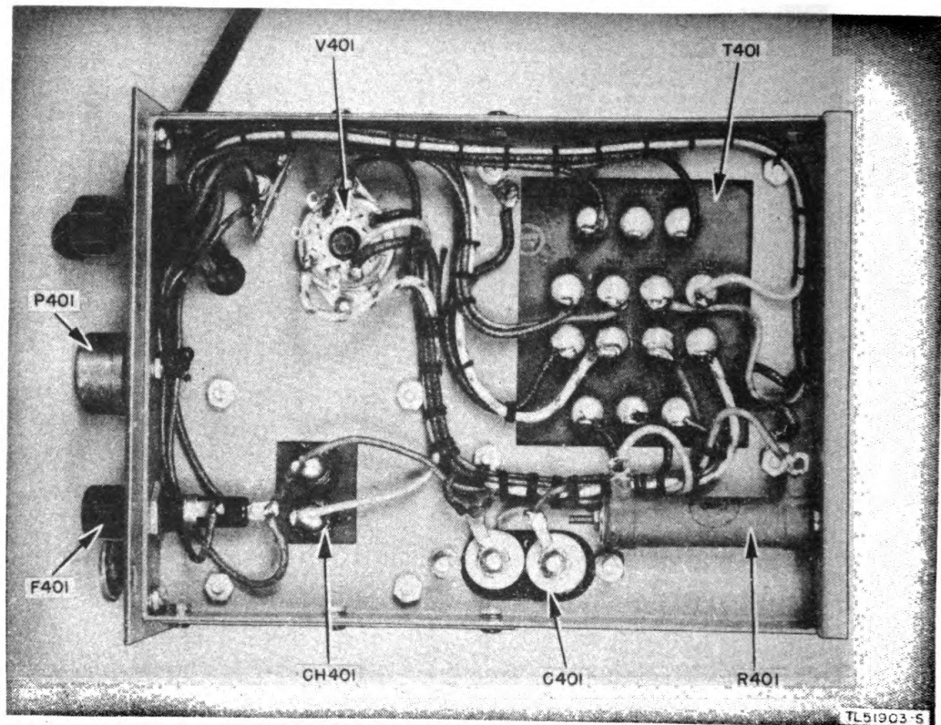
Figure 50. Rectifier power unit, bottom view.
