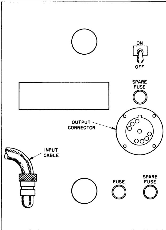
Figure 19. Vibrator power unit, identification of controls.
