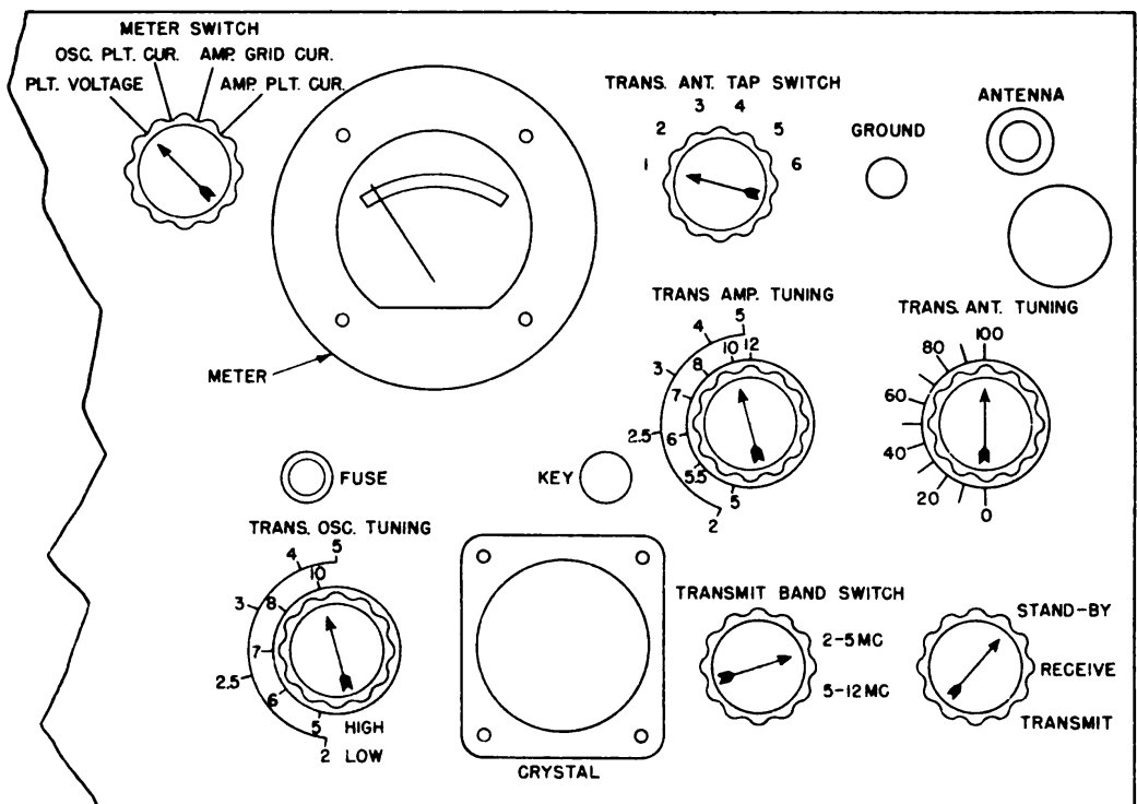
Figure 17. Transmitter section, identification of controls.
