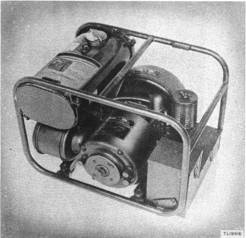
Figure 21. Power Unit PE-214-B.
