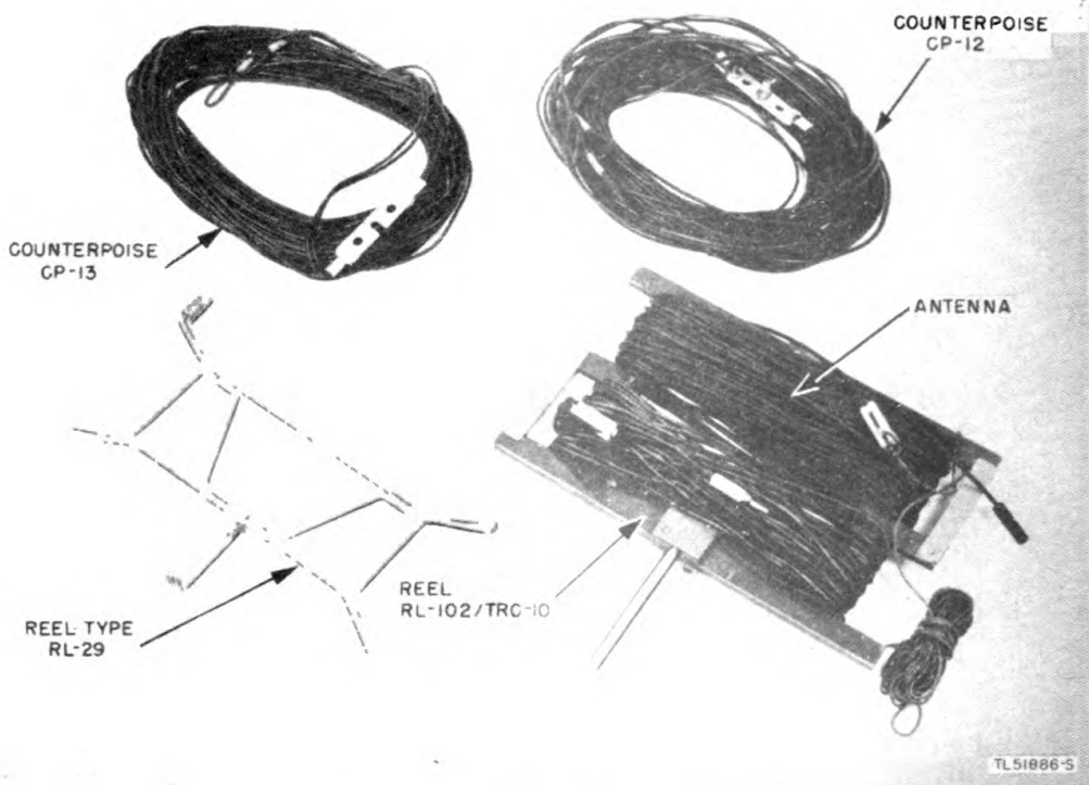
Figure 9. Antenna and counterpoise.
