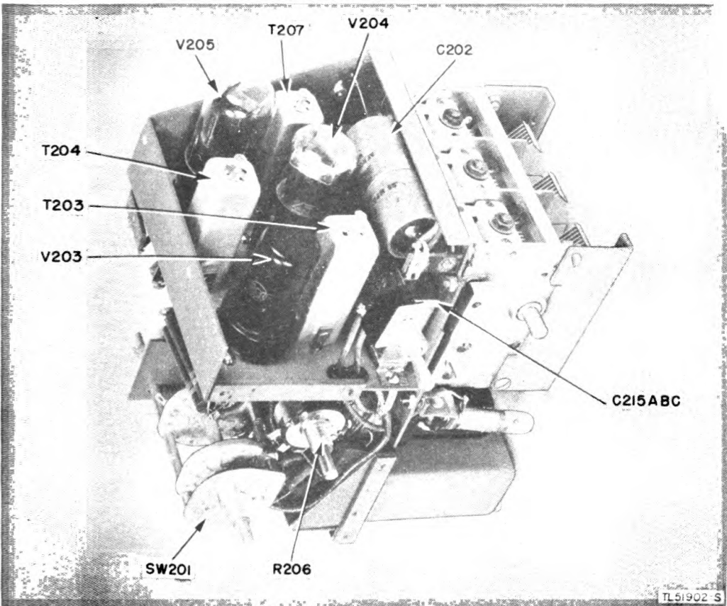
Figure 44. Receiver section, bottom view.
