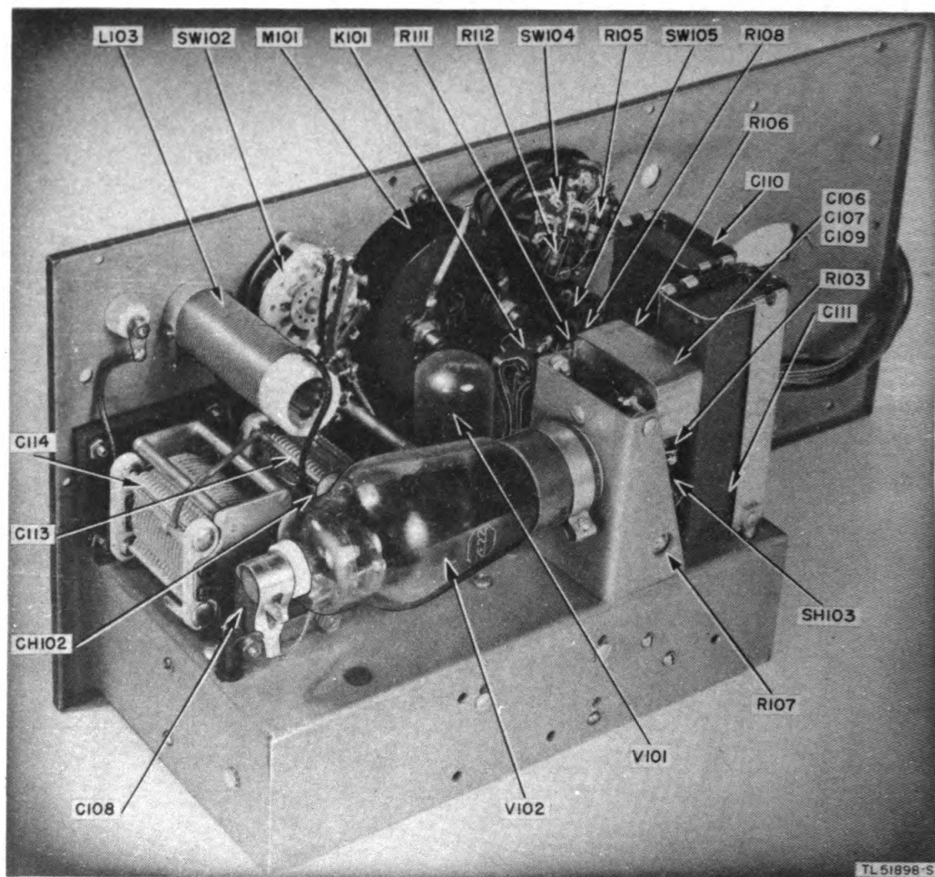
Figure 47. Transmitter section, rear view.
