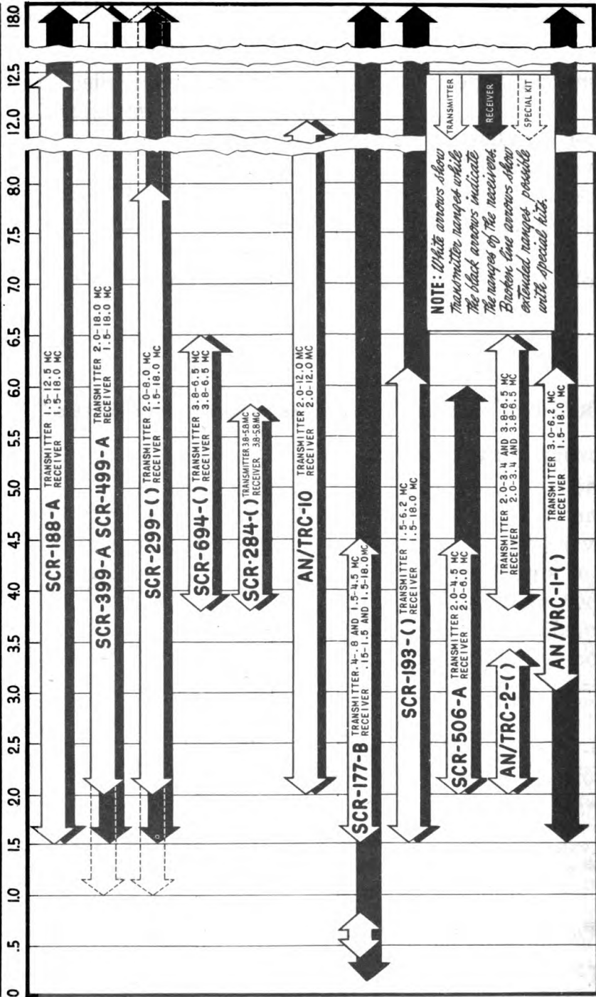
Figure 3. Frequency spectrum chart.
