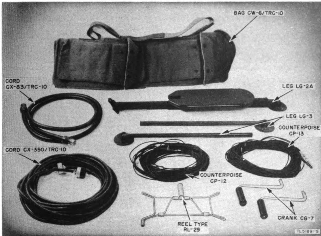
Figure 12. Bag CW-6/TRC-10 and contents.
