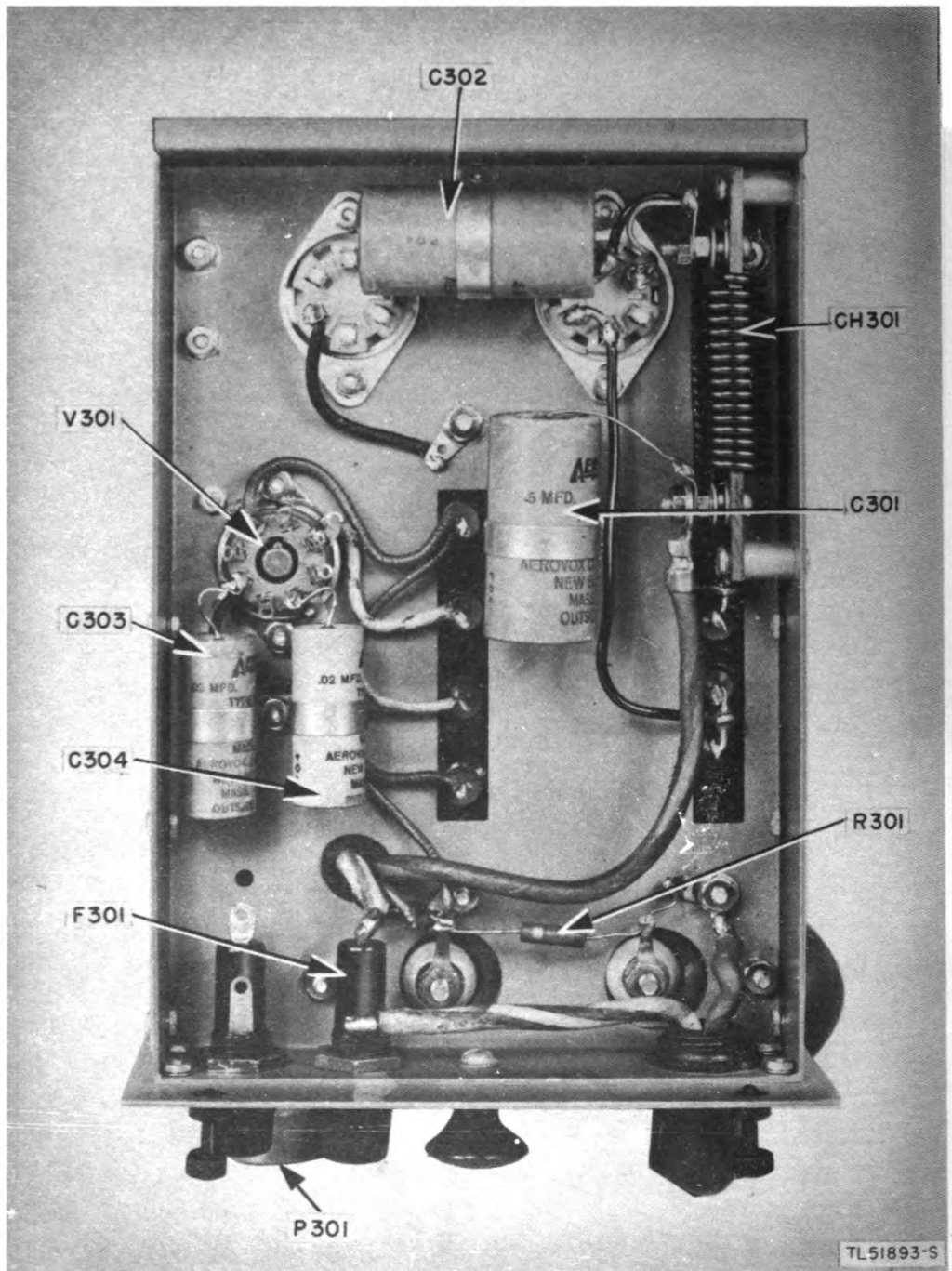
Figure 52. Vibrator power unit, bottom view.
