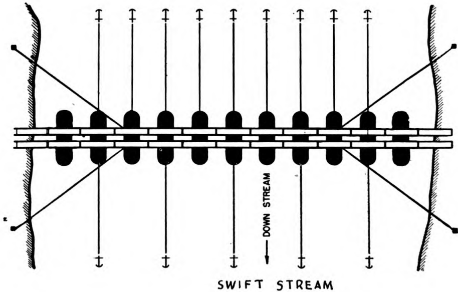
Figure 16. Anchor Spacing.
