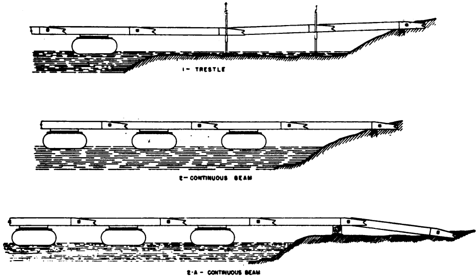
Figure 2. Typical Shore Connection.
