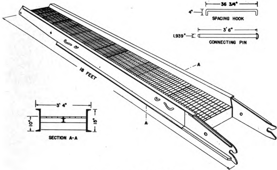
Figure 7. Steel treadway.
