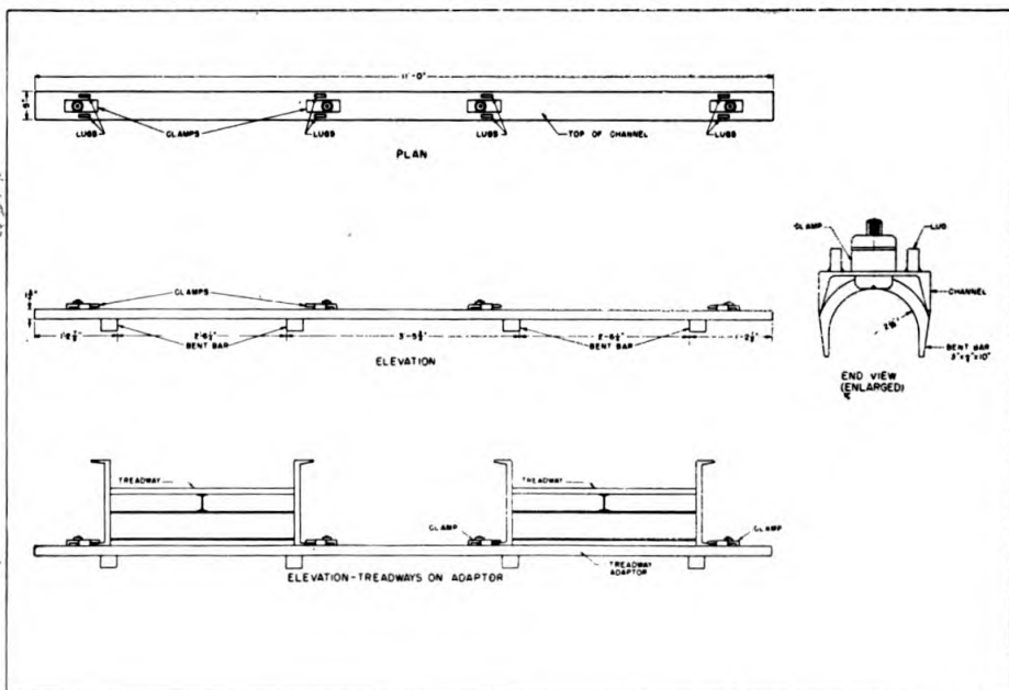
Figure 6. Treadway adaptor.
