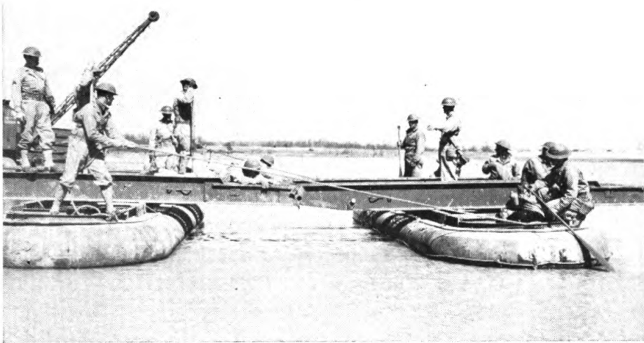
Figure 24. Assembling a ponton section into the bridge.
