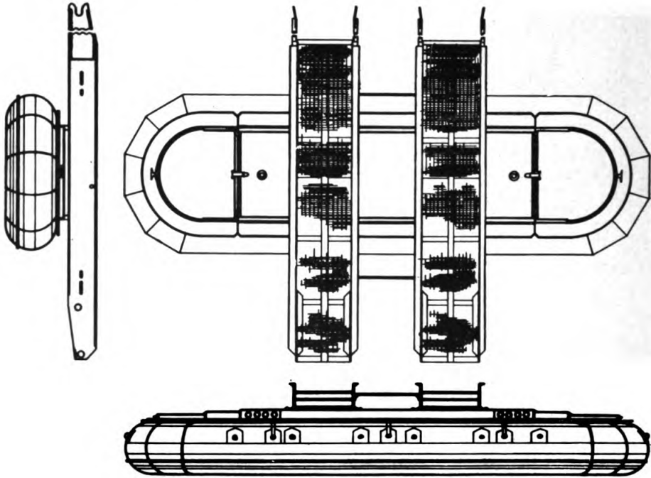
Figure 23. Ponton Section.
