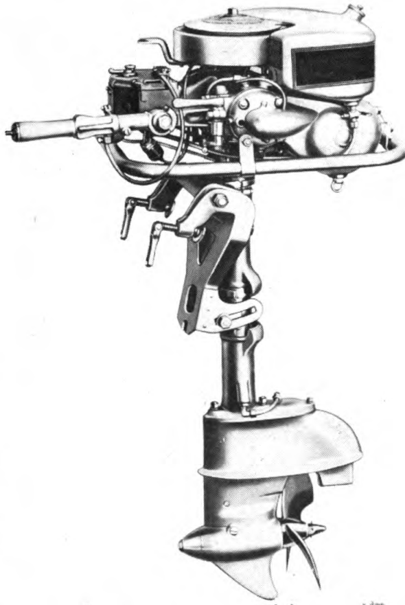
Figure 13. 22-HP Outboard Motor.
