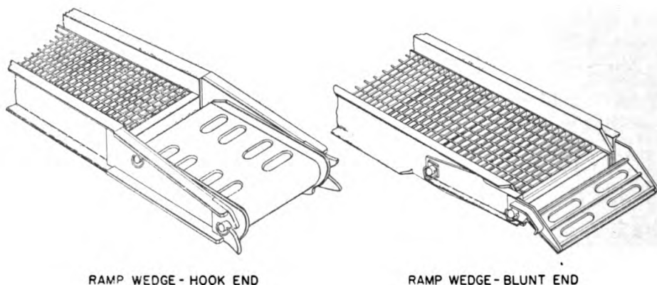
Figure 9. Treadway wedges.
