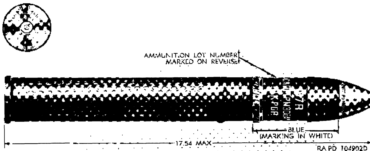
Figure 8. Cartridge, 57 millimeter: TP, MS06A1, w/fuze, PD, M503 or M503A1.
