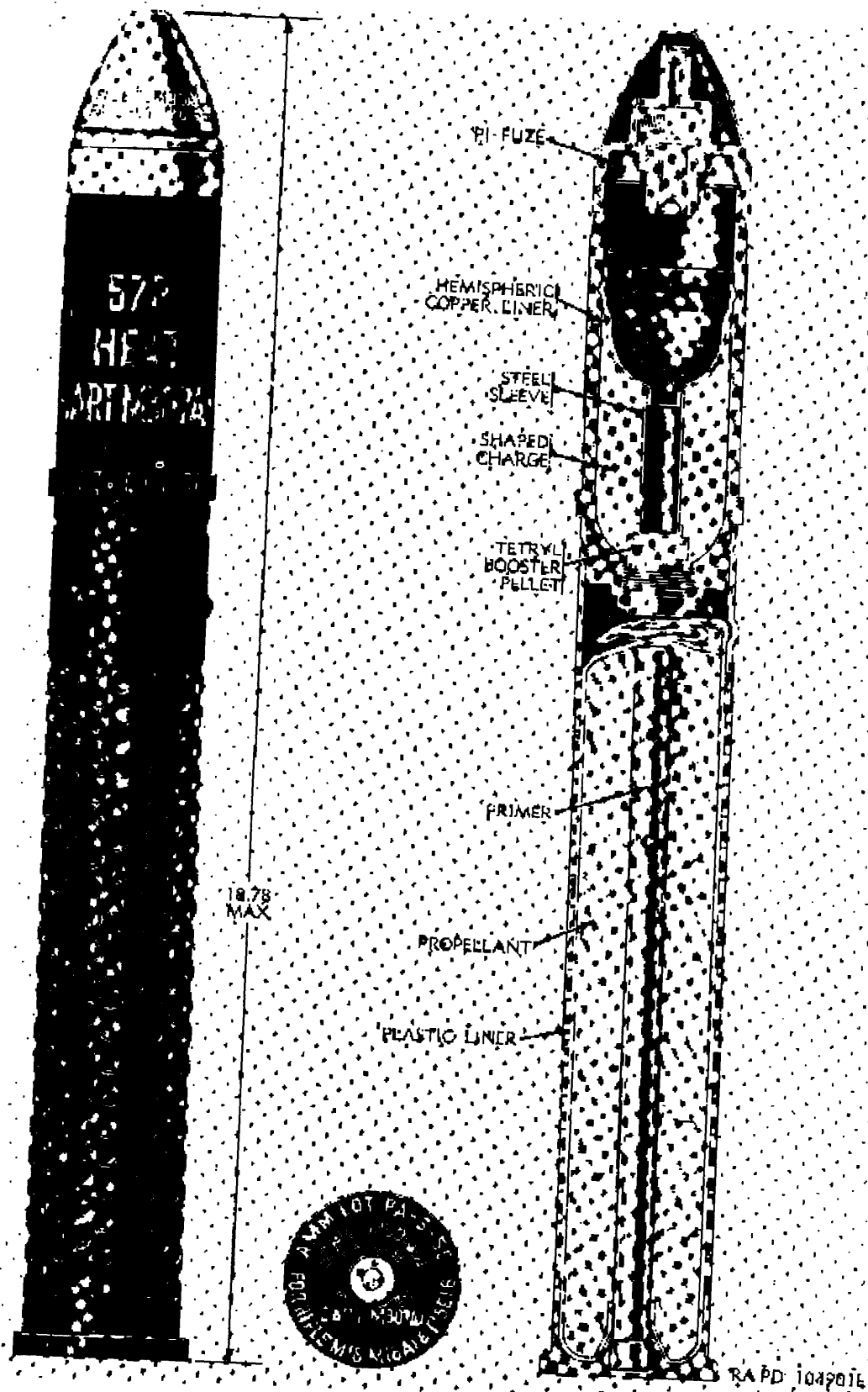
Figure 8. Cartridge, 57 millimeter: HE, AT, M307A1, w/ fuze, PI, M80 or M80A1 (color).
