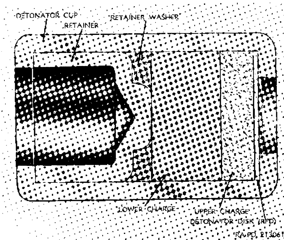
Figure 19. Typical detonator.
