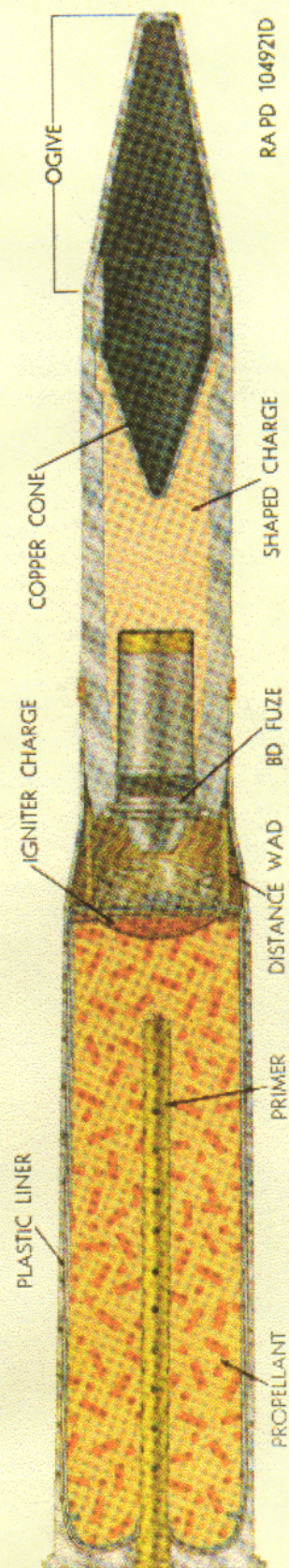
Figure 10. Cartridge, 75 millimeter: HE, AT-T, M810A1, as/foze, BD, M91A1.
