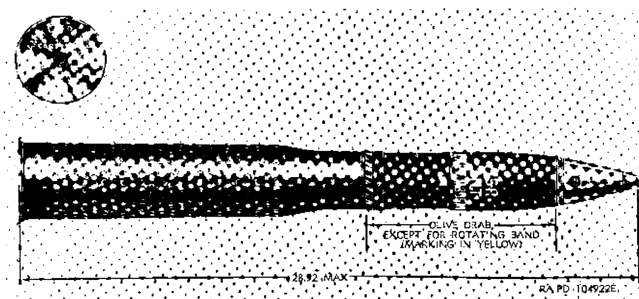
Figure 9. Cartridge, 75 millimeter: HE, M310A1, w/fuze, PD, M51A5, 0.05-sec delay.
