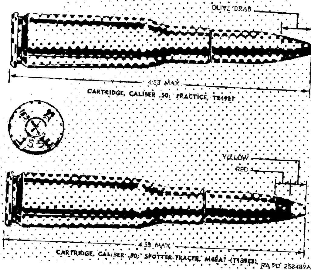
Figure 17. Cartridges for caliber .50 spotting rifle M57.
