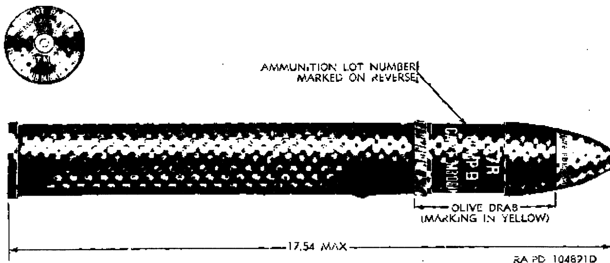
Figure 5. Cartridge, 57 millimeter: HE, M306A1, w/fuze, PD, M503A1.
