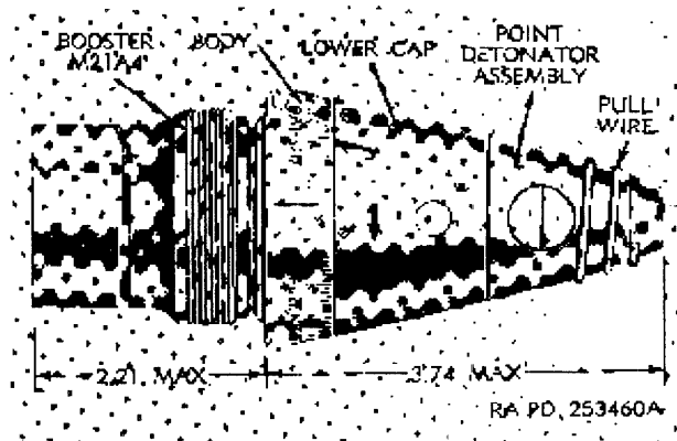
Figure 23. Fuze, MTSQ: M500A1
