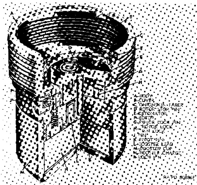
Figure 29. Booster, M21A4.
