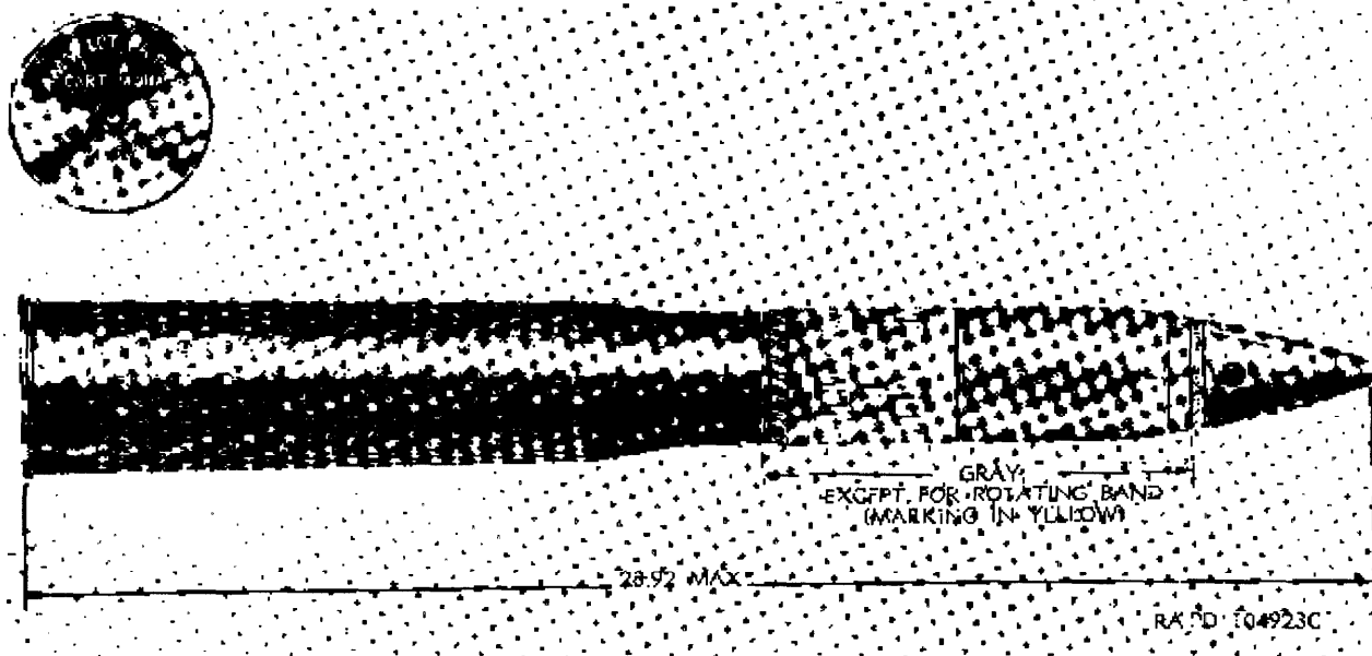
Figure 12. Cartridge, 75 millimeter: smoke, WP, M811A1, w/fuze, PD, M48A3, 0.05-sec delay.
