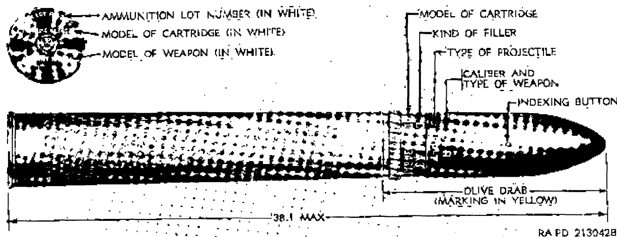
Figure 14. Cartridge, 106 millimeter: HEP T, M348A1, w/fuze, RD, M91A1.
