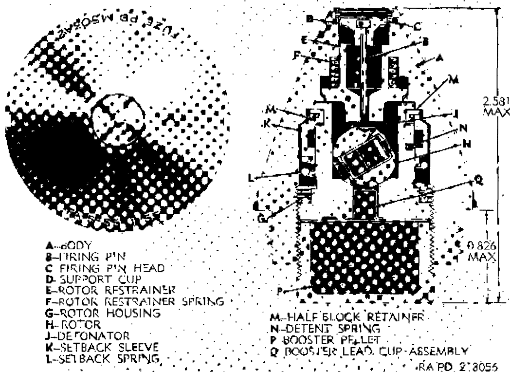
Figure 27. Fuze, PD: M503A2—rotor in unarmed position.
