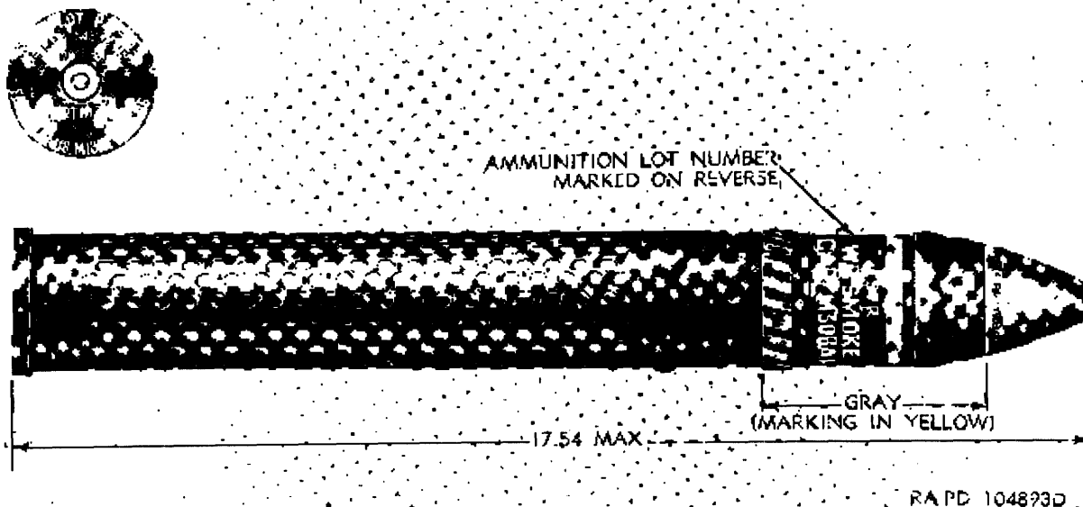
Figure 7. Cartridge, 57 millimeter: smoke, WP, MS08A1, w/fuze, PD, MS08A1.
